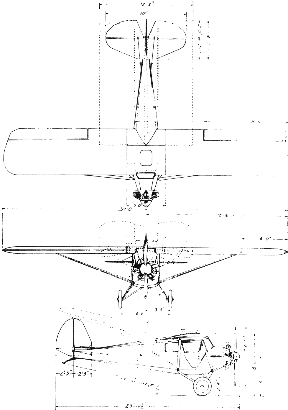
AMERICAN EAGLE AIRCRAFT CORPORATION Kansas City, Kan. WALLACE TOURPLANE 3 AND 4 PLACE ENGINE: KINNER WRIGHT WHIRLWIND 165
