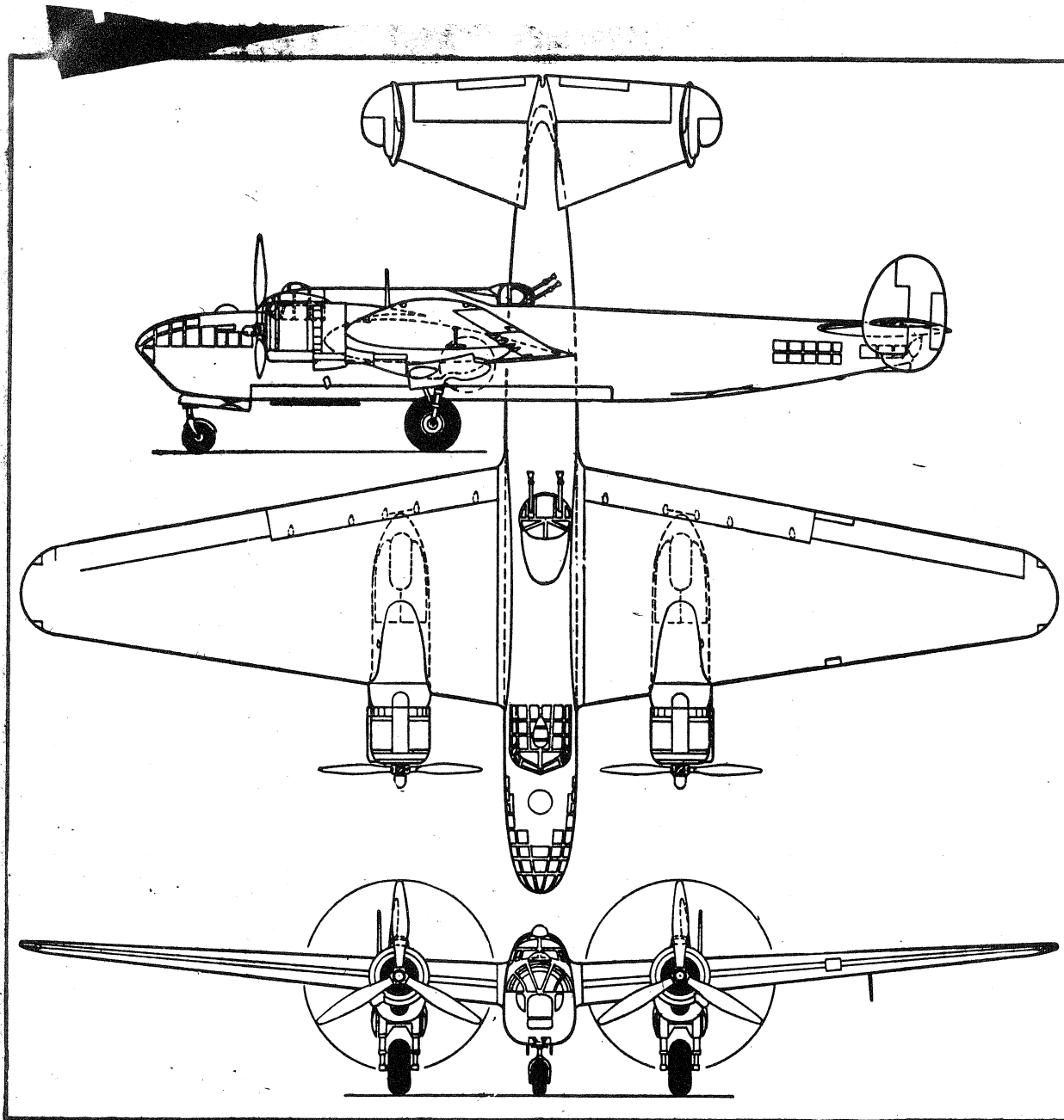
ARMSTRONG WHITWORTH ALBERMARLE , originally designed as a reconnaissance bomber—now glider tug. Span 77 ft; speed 250 mph; 1,590-hp Hercules.
