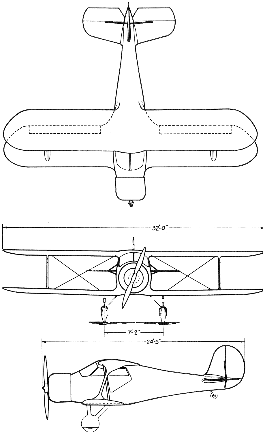
THE BEECH AIRCRAFT COMPANY Wichita, Kans. MODEL B17L — 4 PLACE ENGINE: WRIGHT WHIRLWIND
