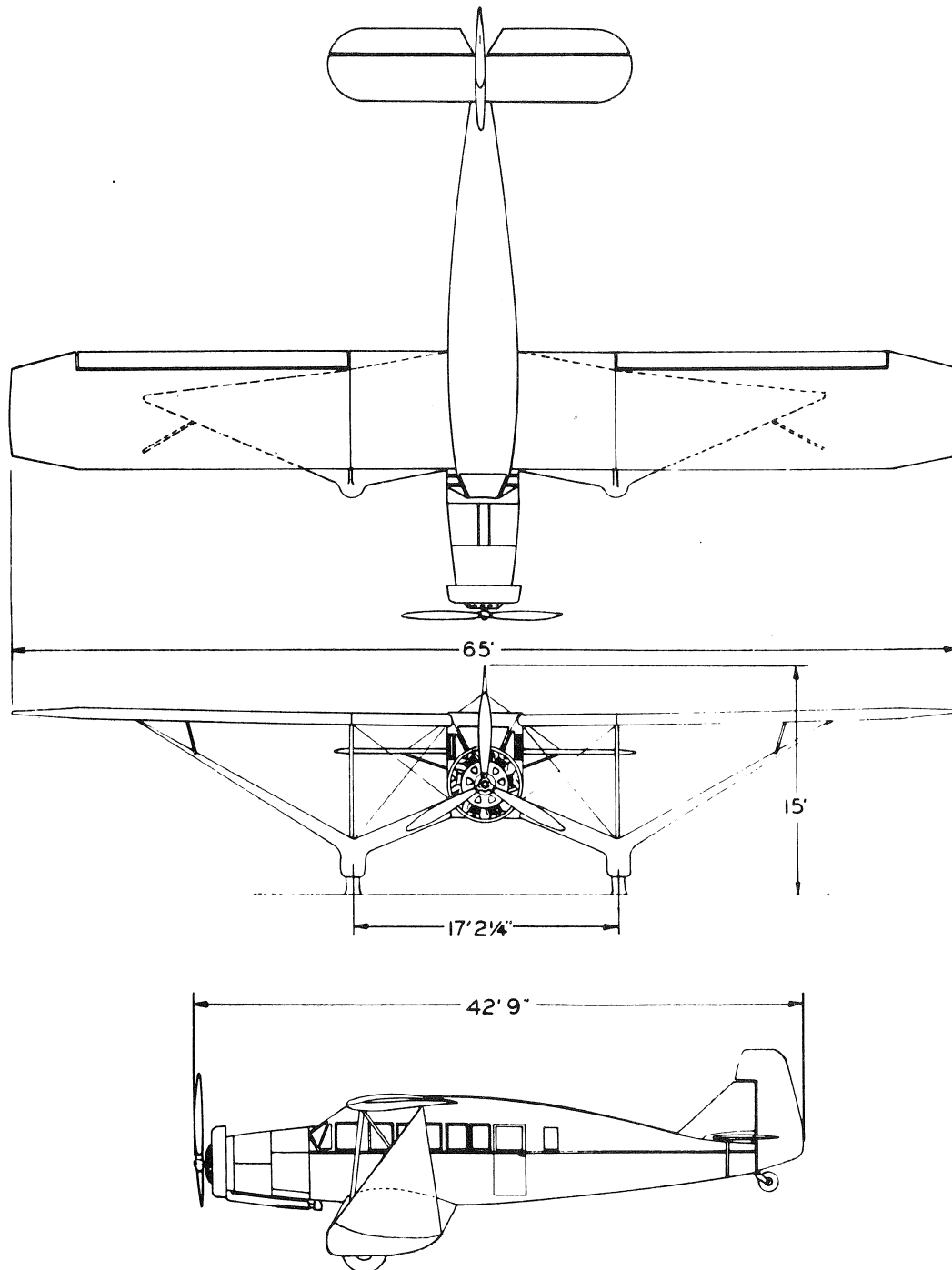
BELLANCA AIRCRAFT CORPORATION New Castle, Del. AIRCUISER — 12-15 PLACE ENGINE: WRIGHT CYCLONE PRATT & WHITNEY HORNET
