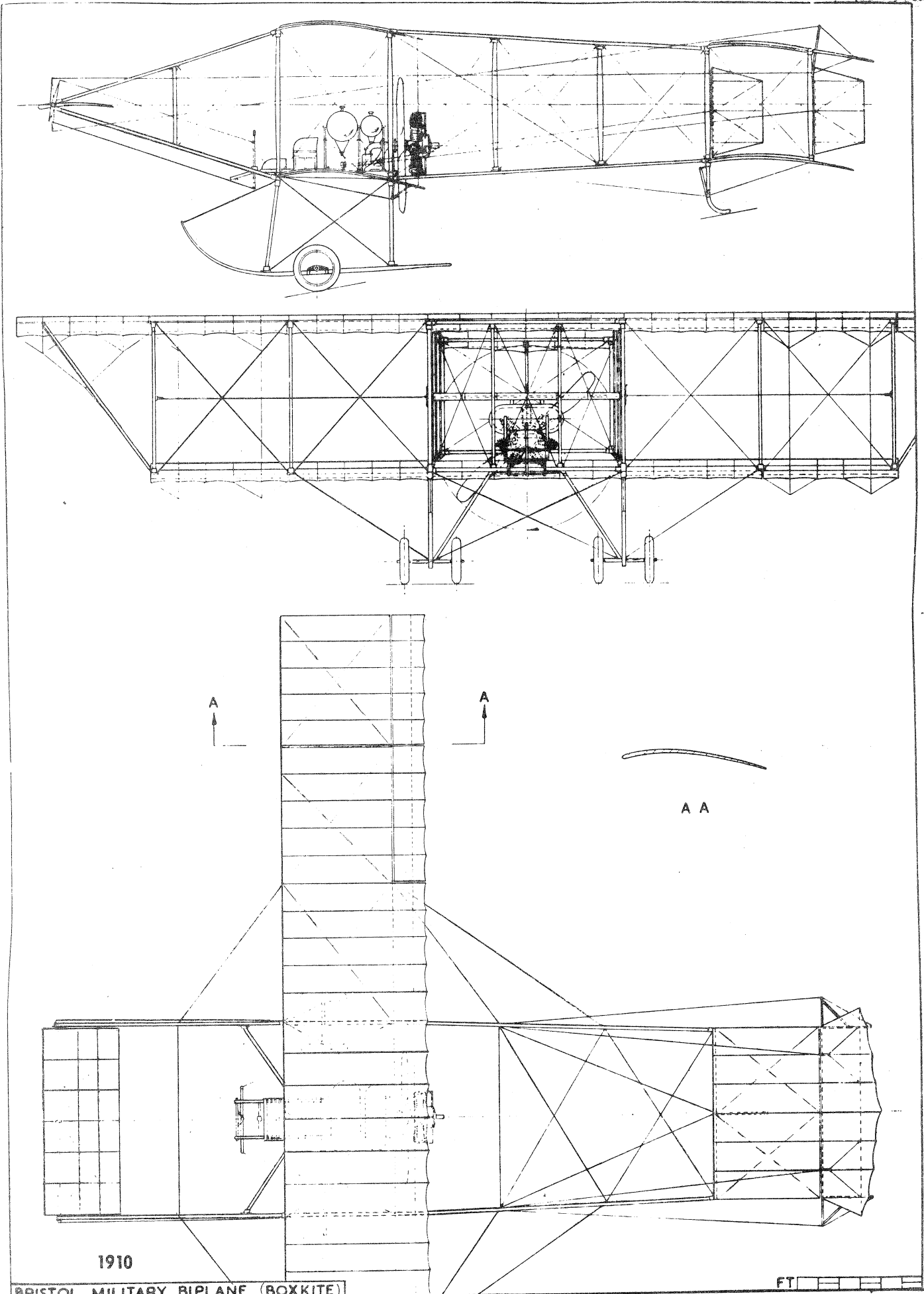
BRISTOL MILITARY BIPLANE (BOXKITE)
