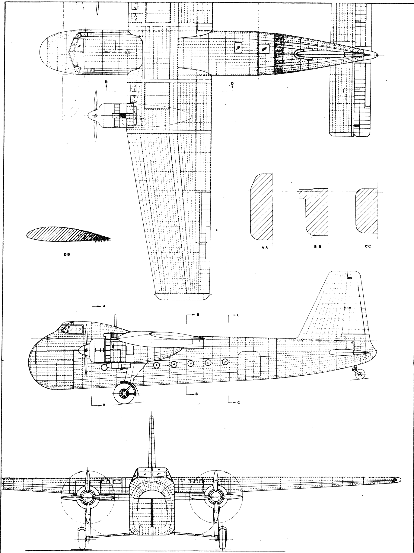
BRISTOL FREIGHTER T.170 1946
