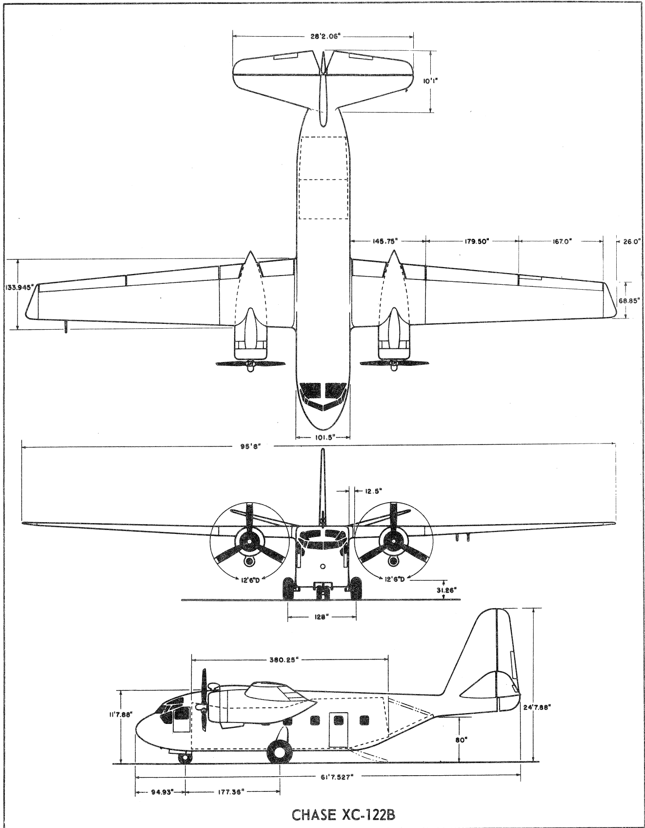
Figure 1-4. Principle Overall Dimensions
