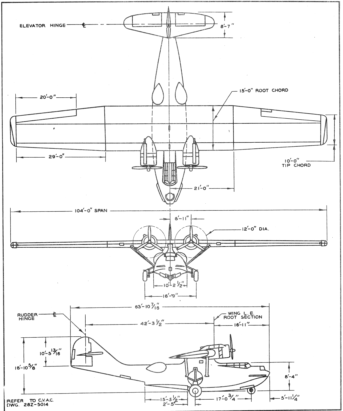
Consolidated Figure C—Three-View Drawing of PB1-5A Airplane
