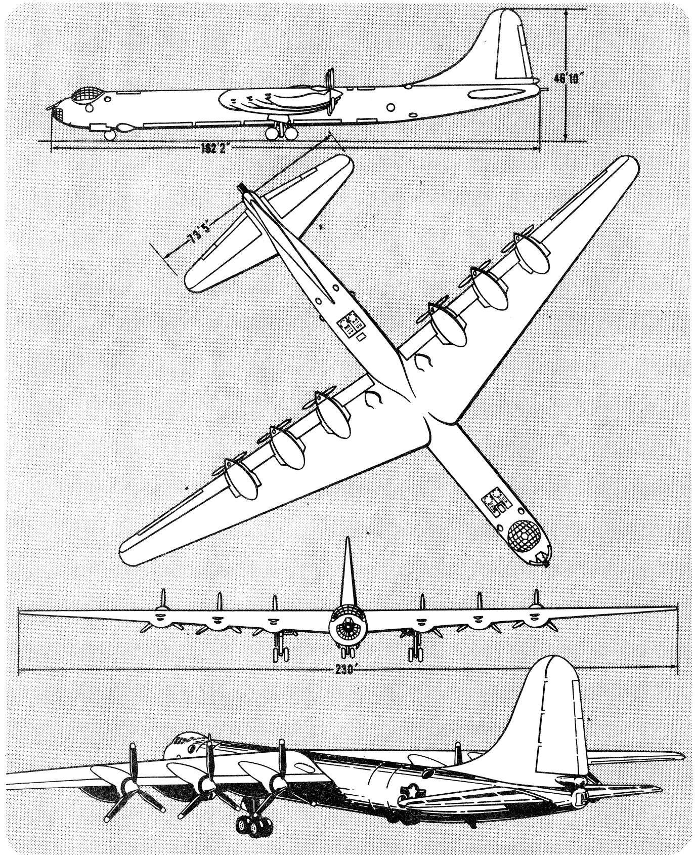
Figure 1. B-36B Airplane Convair
