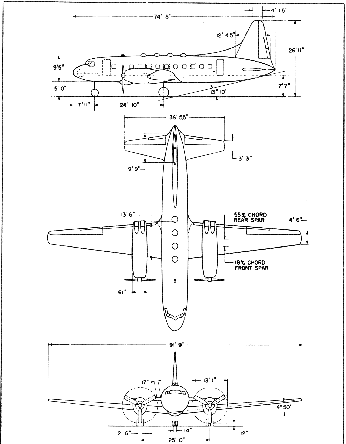
Figure 1-3. Three-View Dimensional Drawing Convair T-29A
