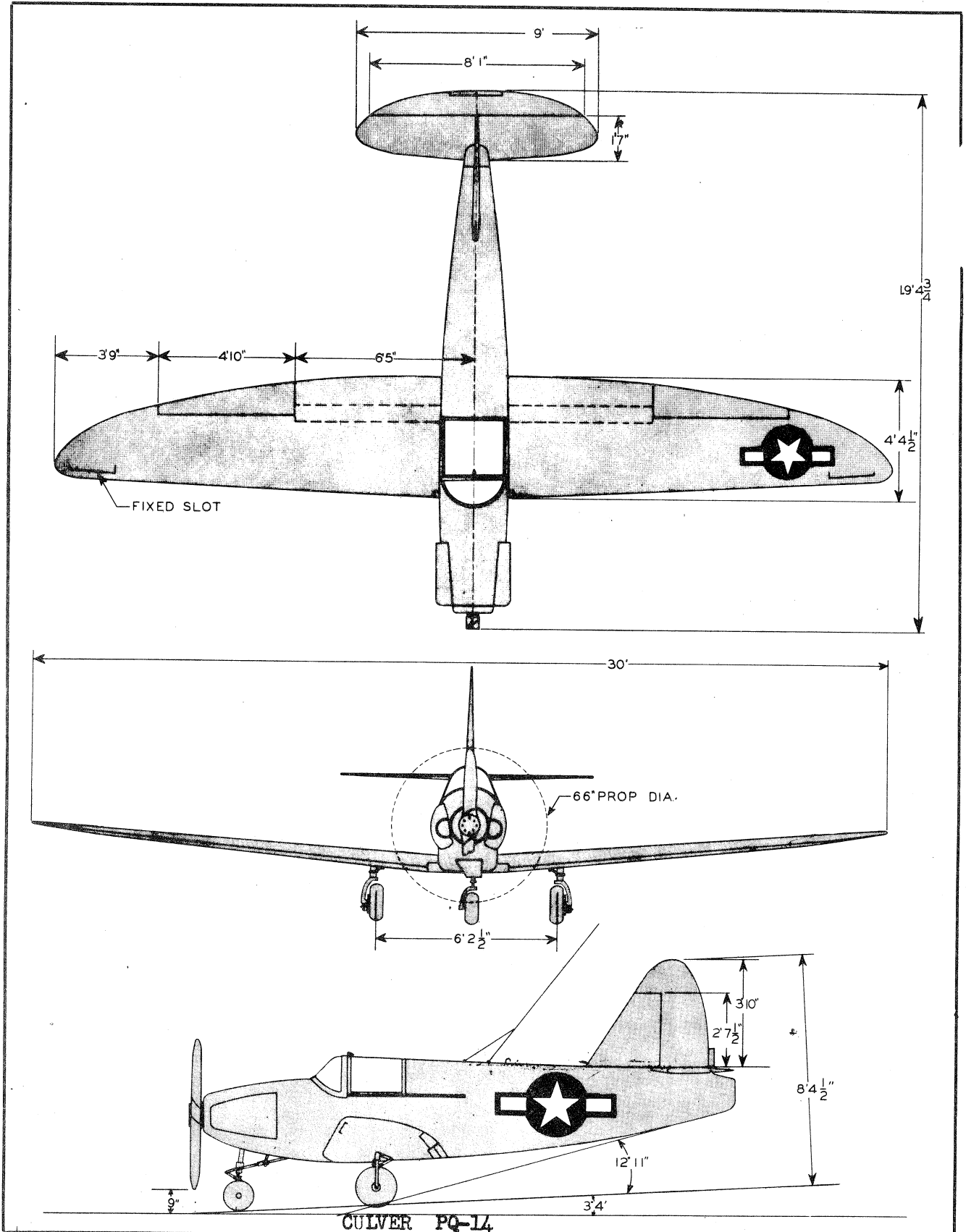
Figure 15—General Dimensions
