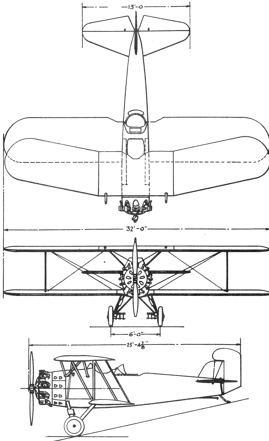
CURTISS AEROPLANE & MOTOR COMPANY, INC. Garden City, L. I., N. Y. FIGHTER XF8C-2 2 PLACE ENGINE: PRATT & WHITNEY WASP
