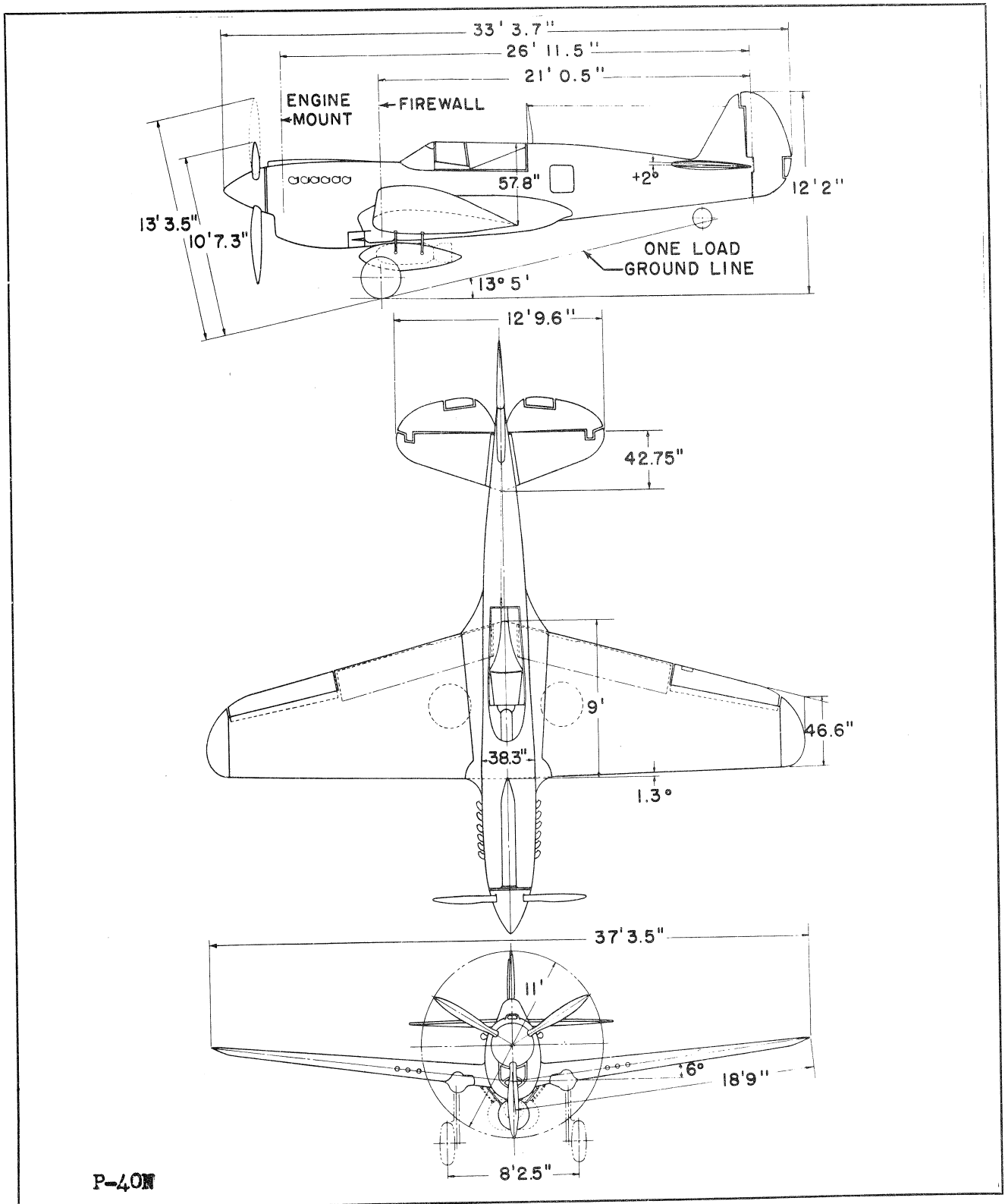
CURTISS P-40N Figure 7—Three View Dimensions
