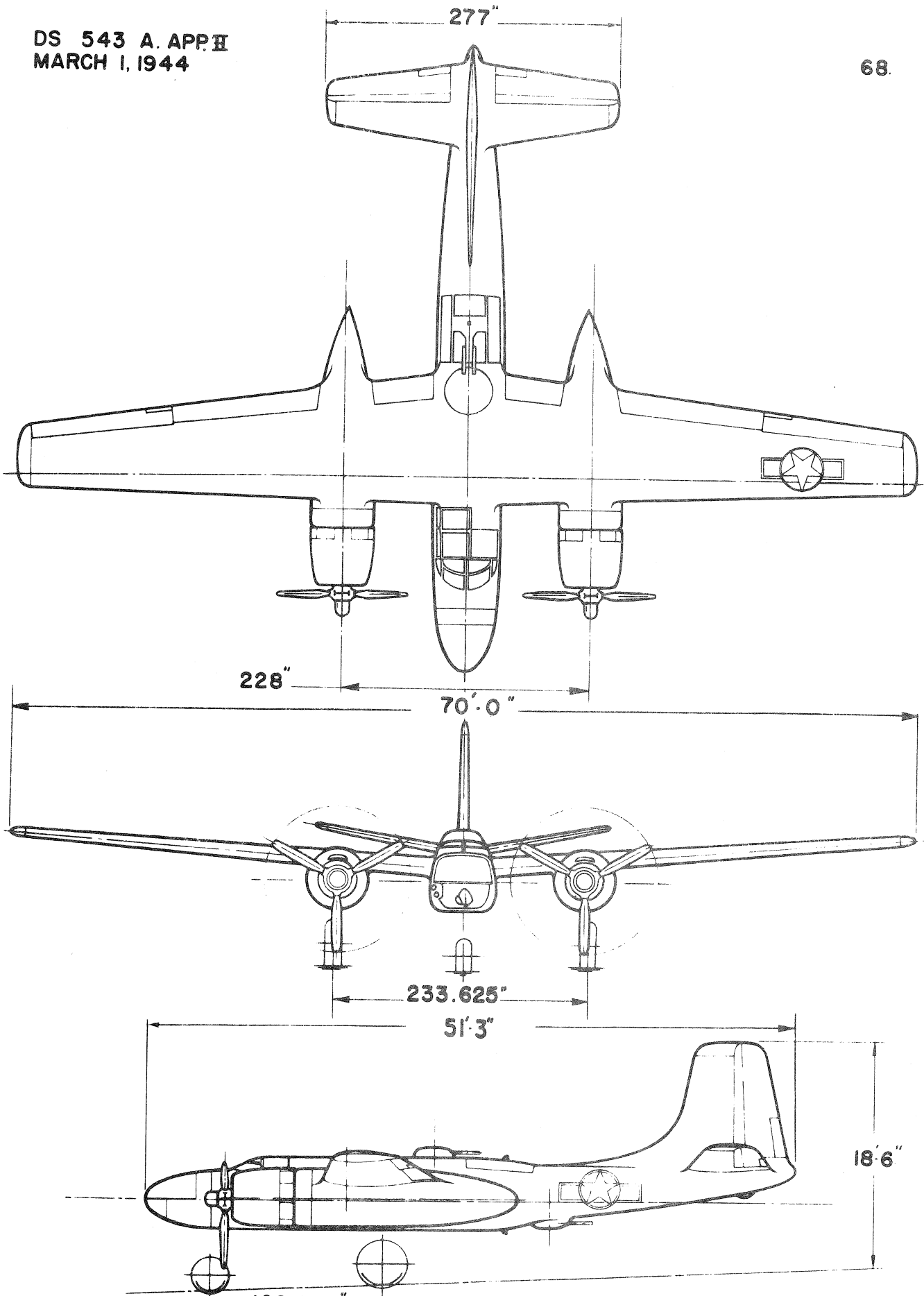
MODEL A-26C ATTACK - BOMBER AIRPLANE
