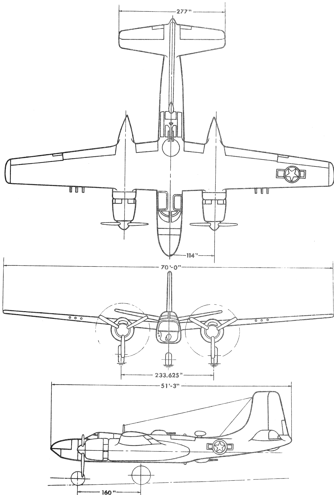
MODEL A-26E ATTACK - BOMBER AIRPLANE
