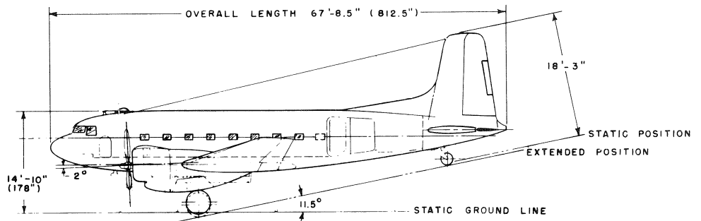
3-VIEW DIAGRAM
