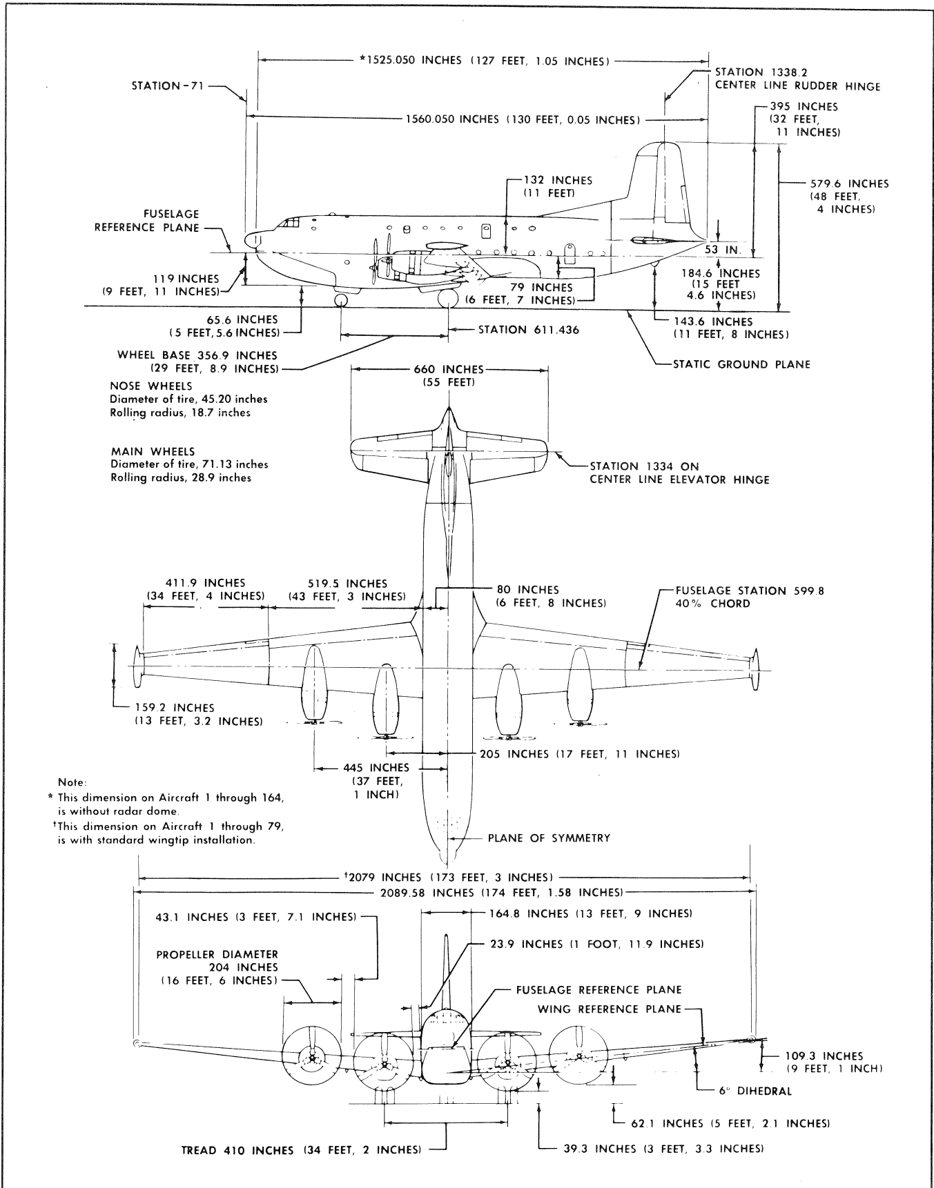
Three-Views of Aircraft
