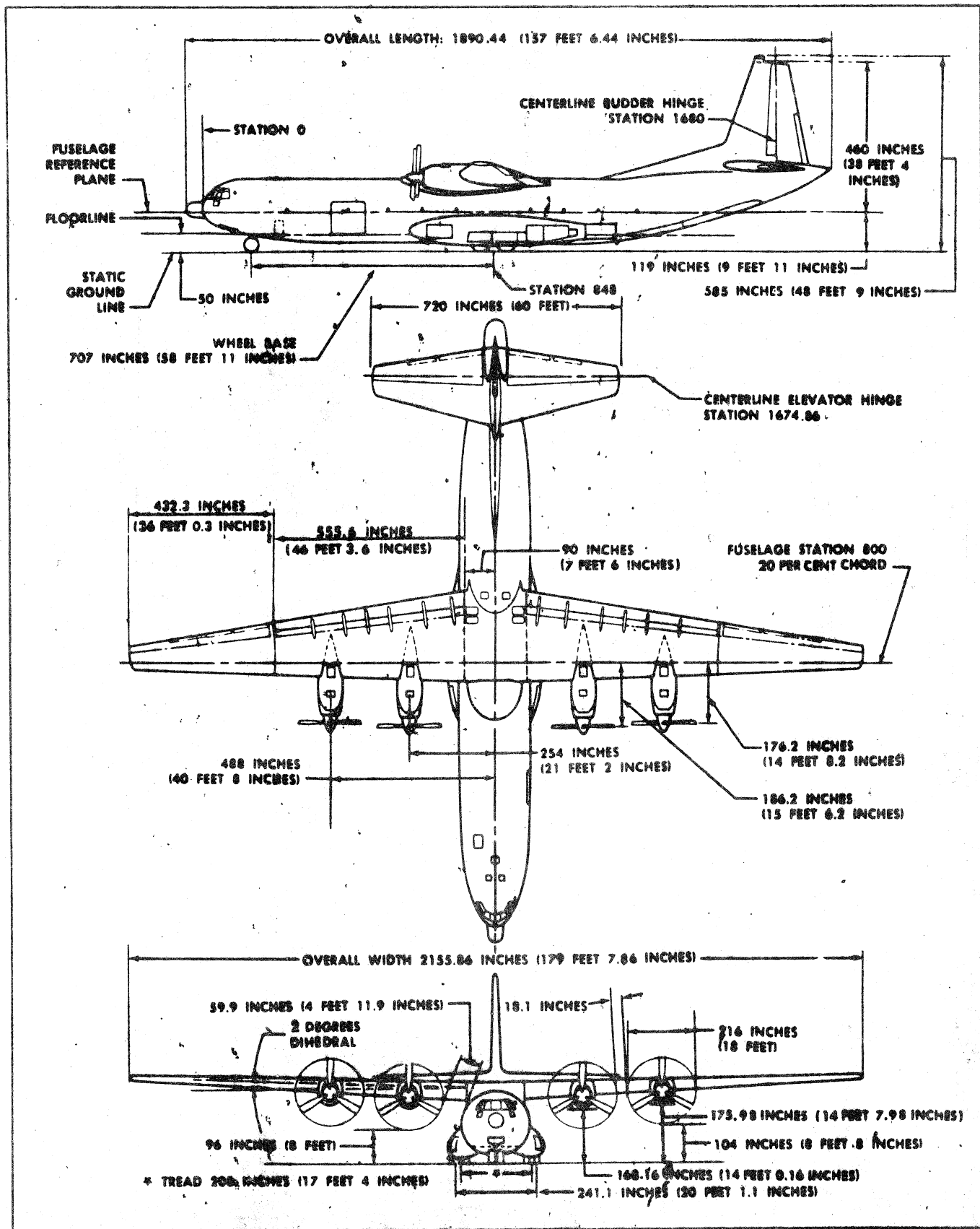
Figure 1-1, Three Views of Airplane
