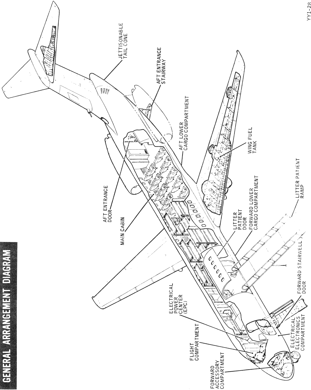
Figure 1-1 C-9A
