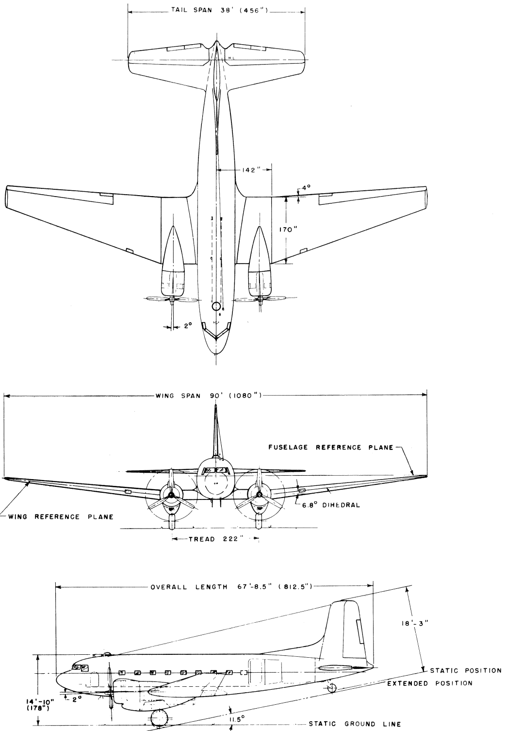
3-VIEW DIAGRAM
