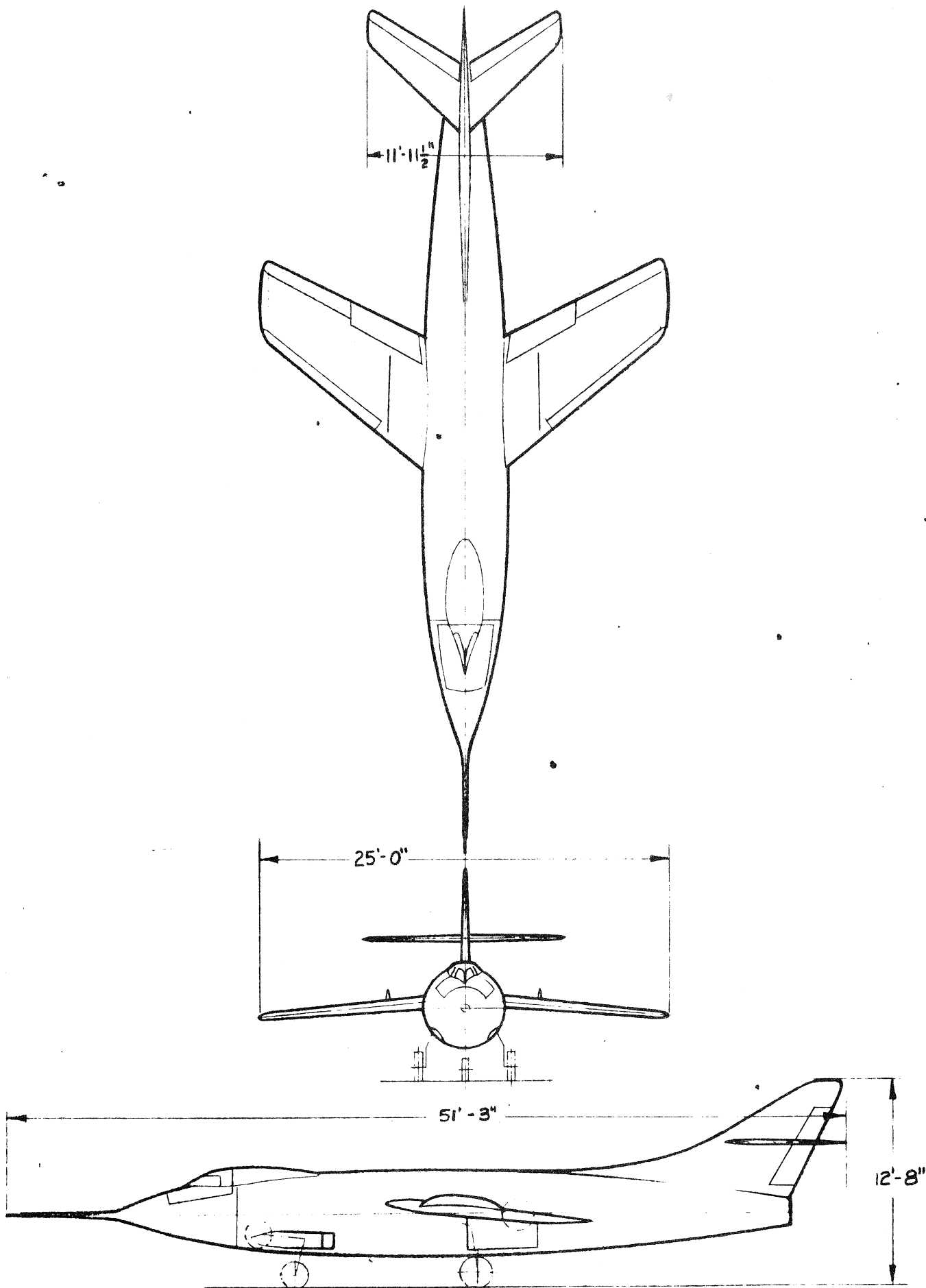
DOUGLAS MODEL D-558-2
