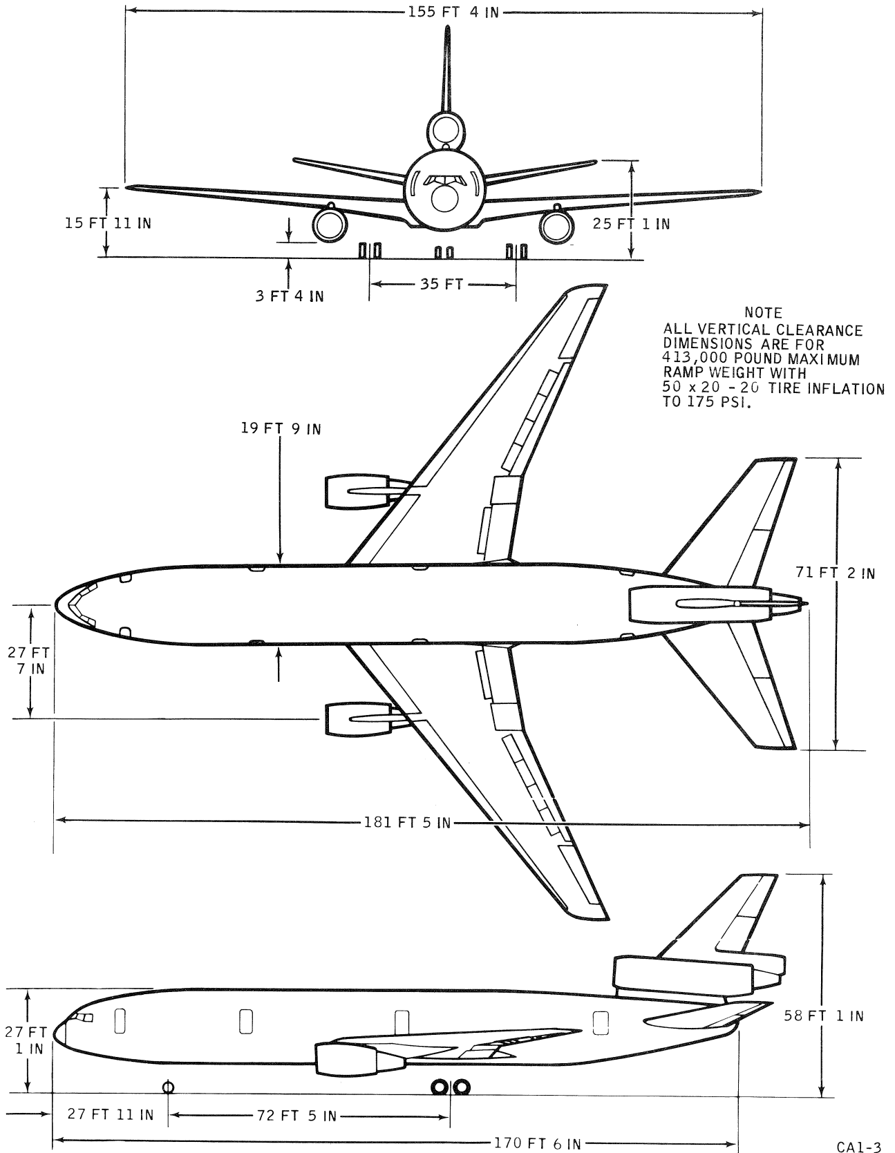
DC-10 SERIES 10
