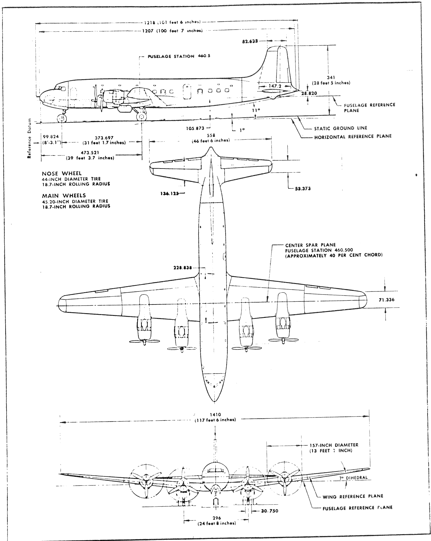
Figure 2 - Three-View of Airplane
