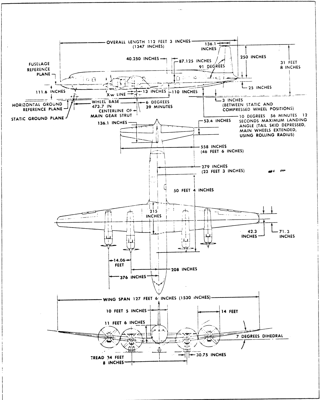
Figure 51-2. Airplane Dimensional Data DC-7C
