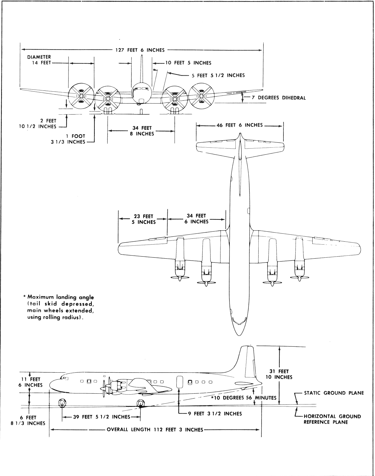
Three-View of Airplane
