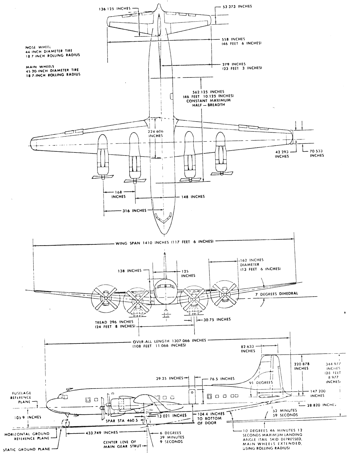
Figure i-4. Airplane Dimensional Data DC-7 & DC-7B
