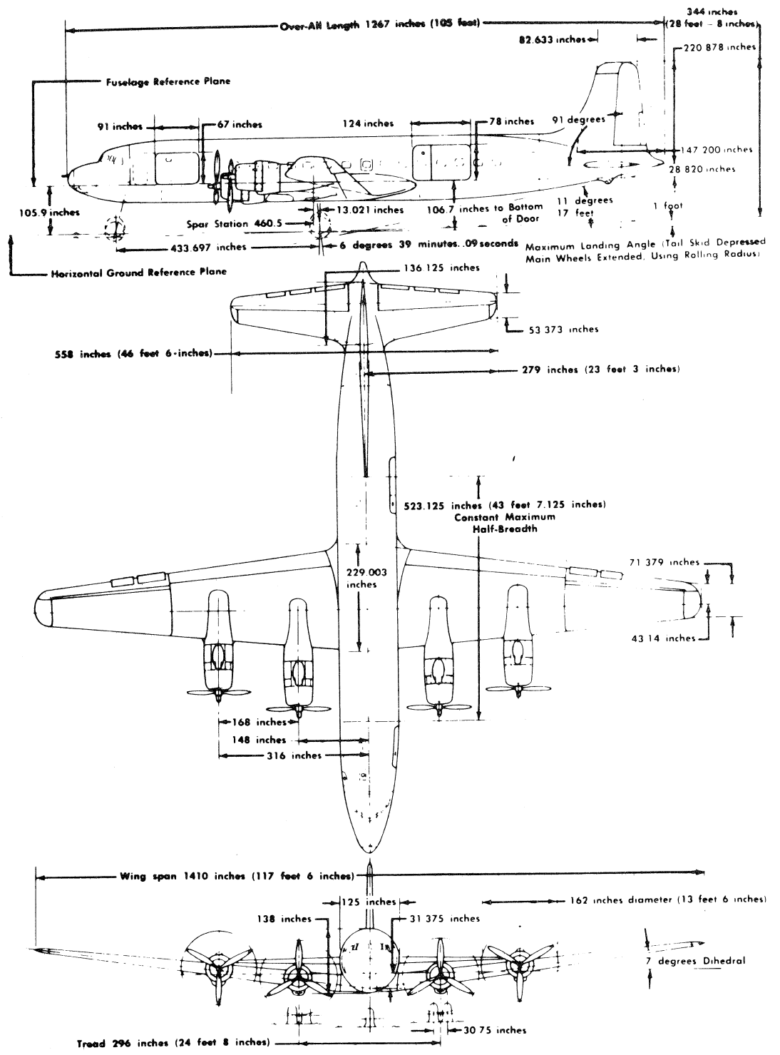
Three-View of Airplane
