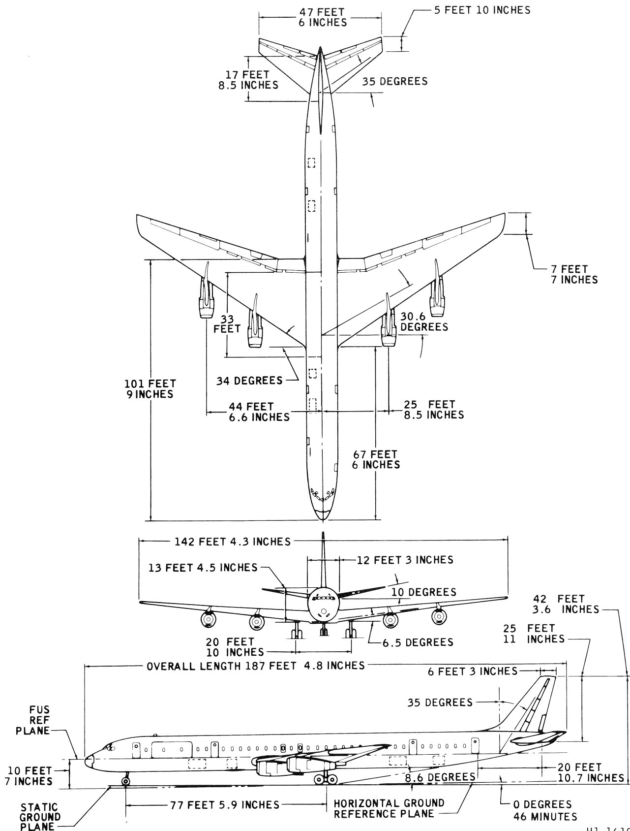
DC-8 SERIES 61
