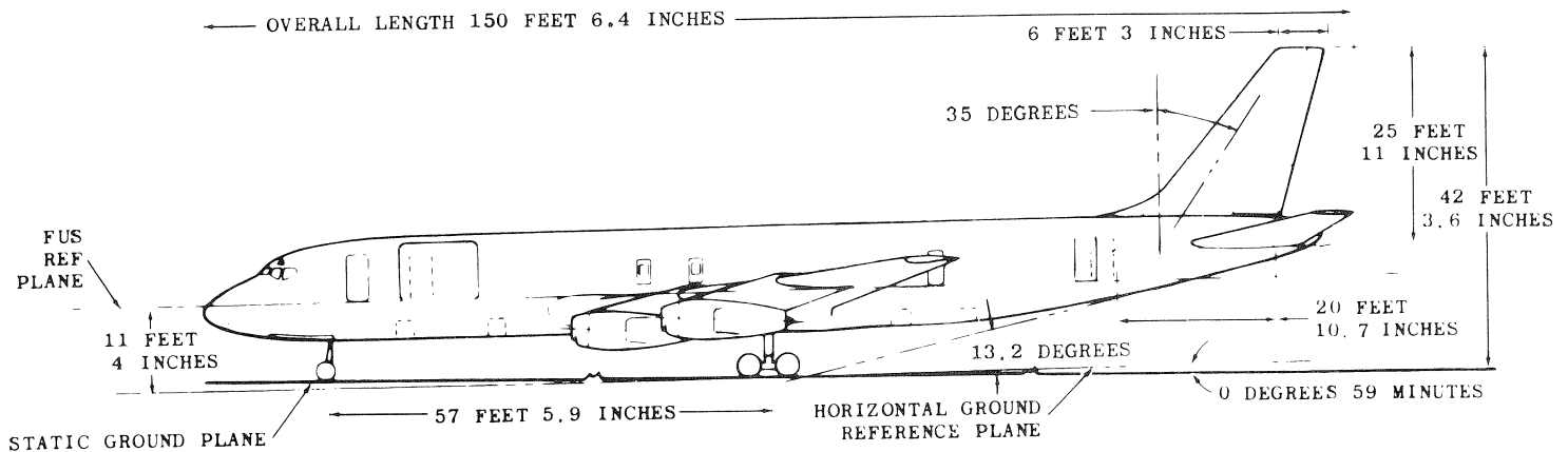
DC-8 SERIES 10 & 50
