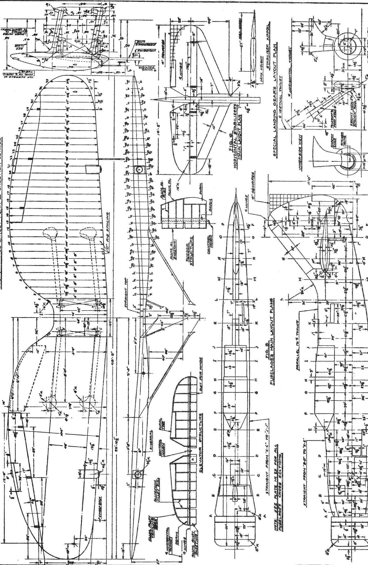
FIG. 4 - WINGS LAYOUT PLAN & ERECTION DETAILS
