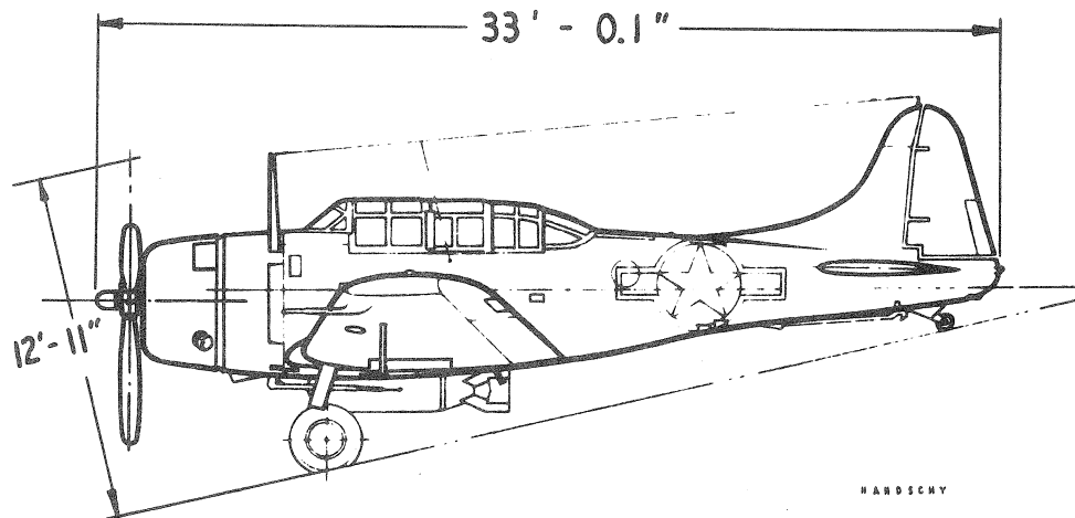
DOUGLAS MODEL SBD-5
