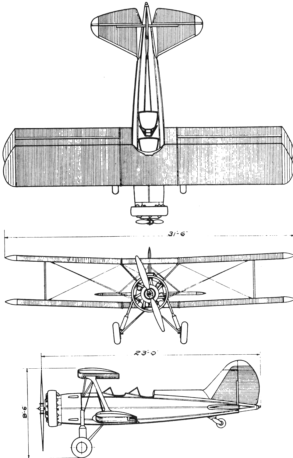
GREAT LAKES AIRCRAFT CORPORATION Cleveland, Ohio MODEL XPT-930 ENGINE: CONTINENTAL
