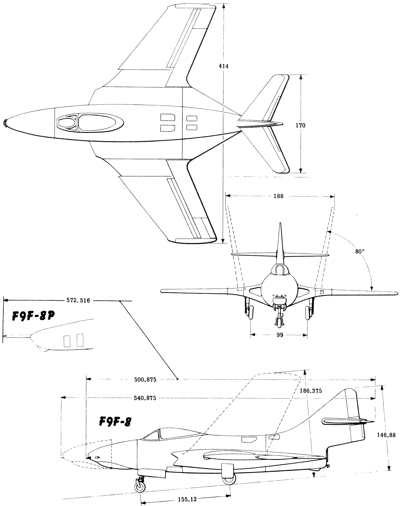
Figure 1-3. Airplane Dimensions (Sheet 2)
