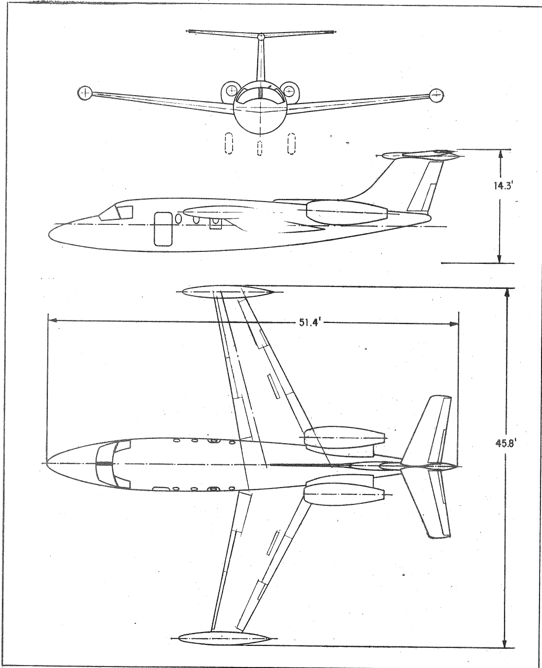
THREE-VIEW of Hamburger Flugzeugbau HFB.320 shows pronounced forward sweep
