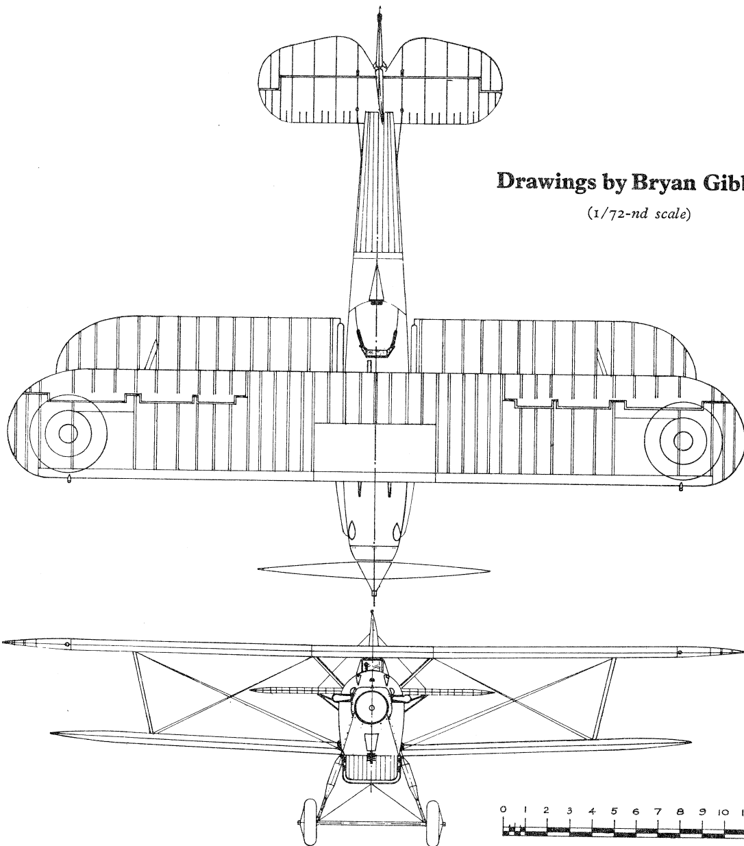
Hawker "Nimrod"
