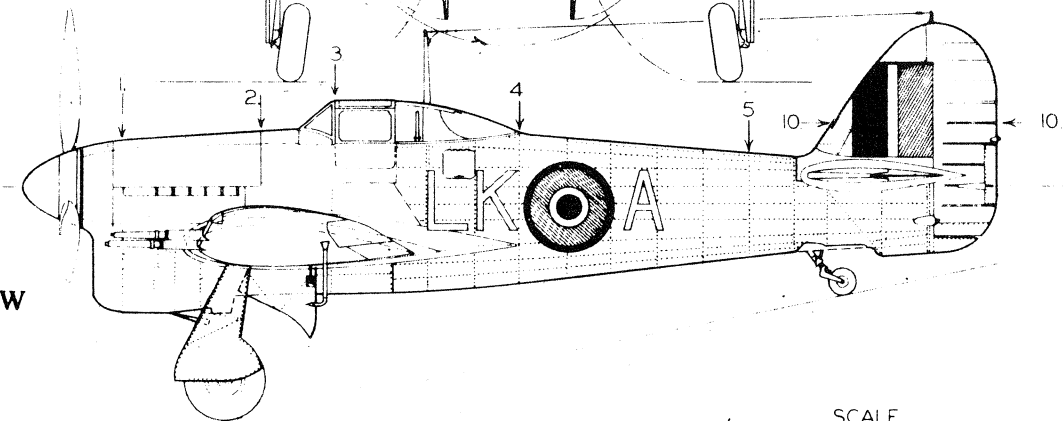
Hawker Tempest IV
