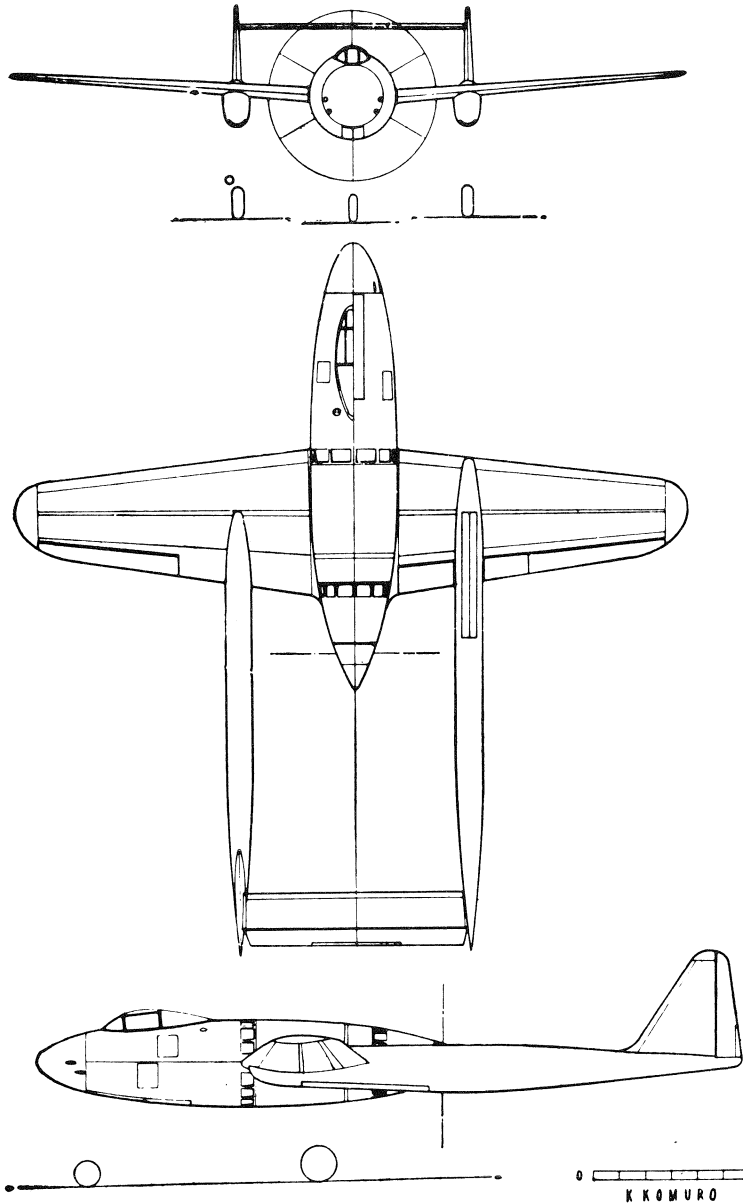
十七試局地戦闘機「閃電」(推定図) EXPERIMENTAL 17-SHI "SENDEN" INTERCEPTOR FIGHTER
