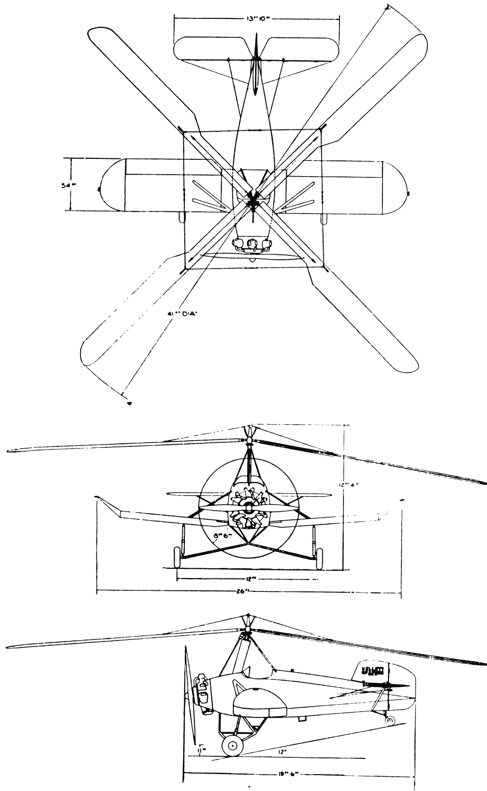
KELLETT AUTOGIRO CORPORATION Philadelphia, Pa. MODEL K-4 — 2 PLACE ENGINE: CONTINENTAL 210 H.P.
