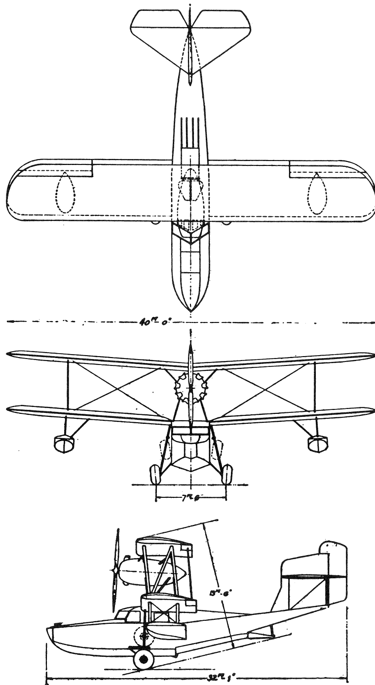
KEYSTONE AIRCRAFT CORPORATION Bristol, Pa. COMMUTER — 4 PLACE ENGINE: WRIGHT WHIRLWIND 330
