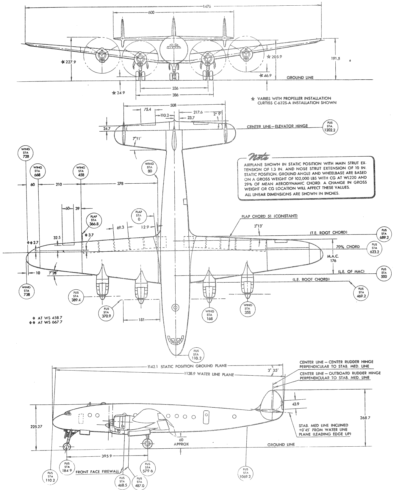
LOCKHEED C-121A & B Figure 1-2 — General Dimensions
