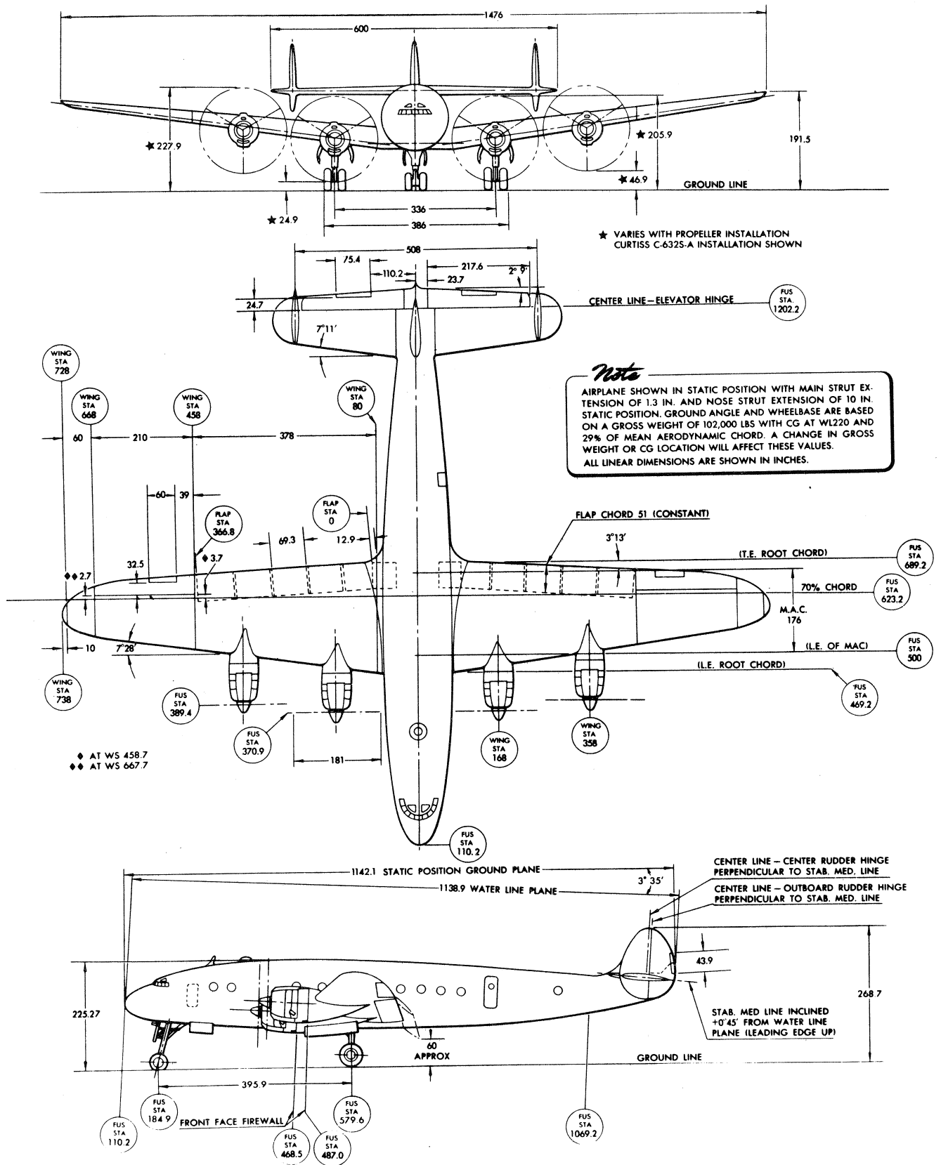
Lockheed C-69
