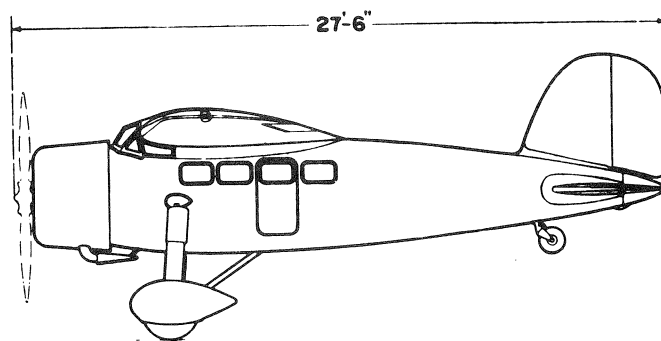
LOCKHEED AIRCRAFT CORPORATION Burbank, Calif. VEGA — 7 PLACE ENGINE: PRATT & WHITNEY WASP SC-1
