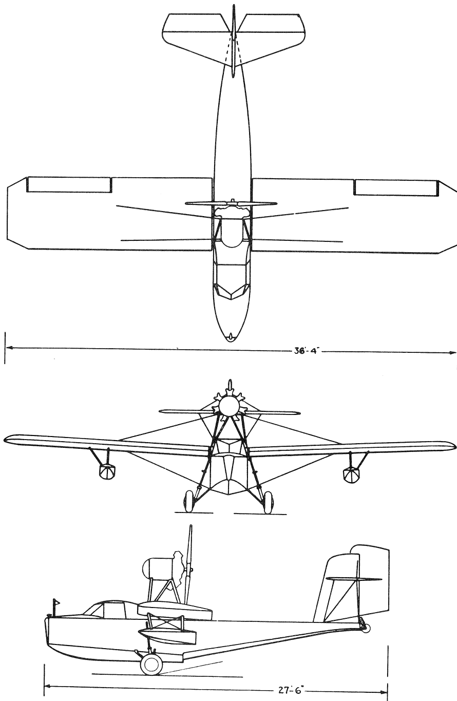
GROVER LOENING AIRCRAFT COMPANY, INC. Garden City, L. I., N. Y. DUCKLING — 2 PLACE ENGINE: WARNER SCARAB
