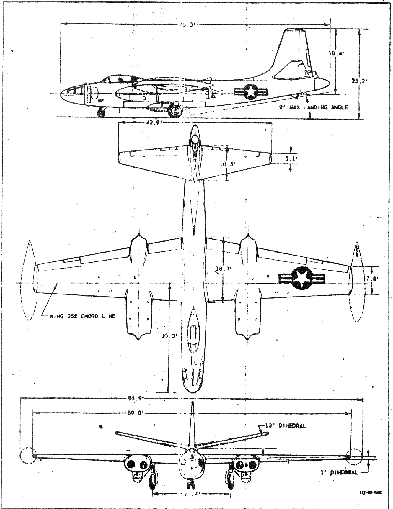
Figure 1-1. Airplane Dimensions
