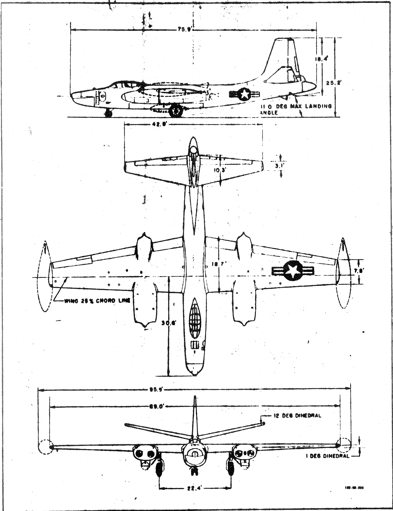
Figure 1-1. Airplane Dimensions
