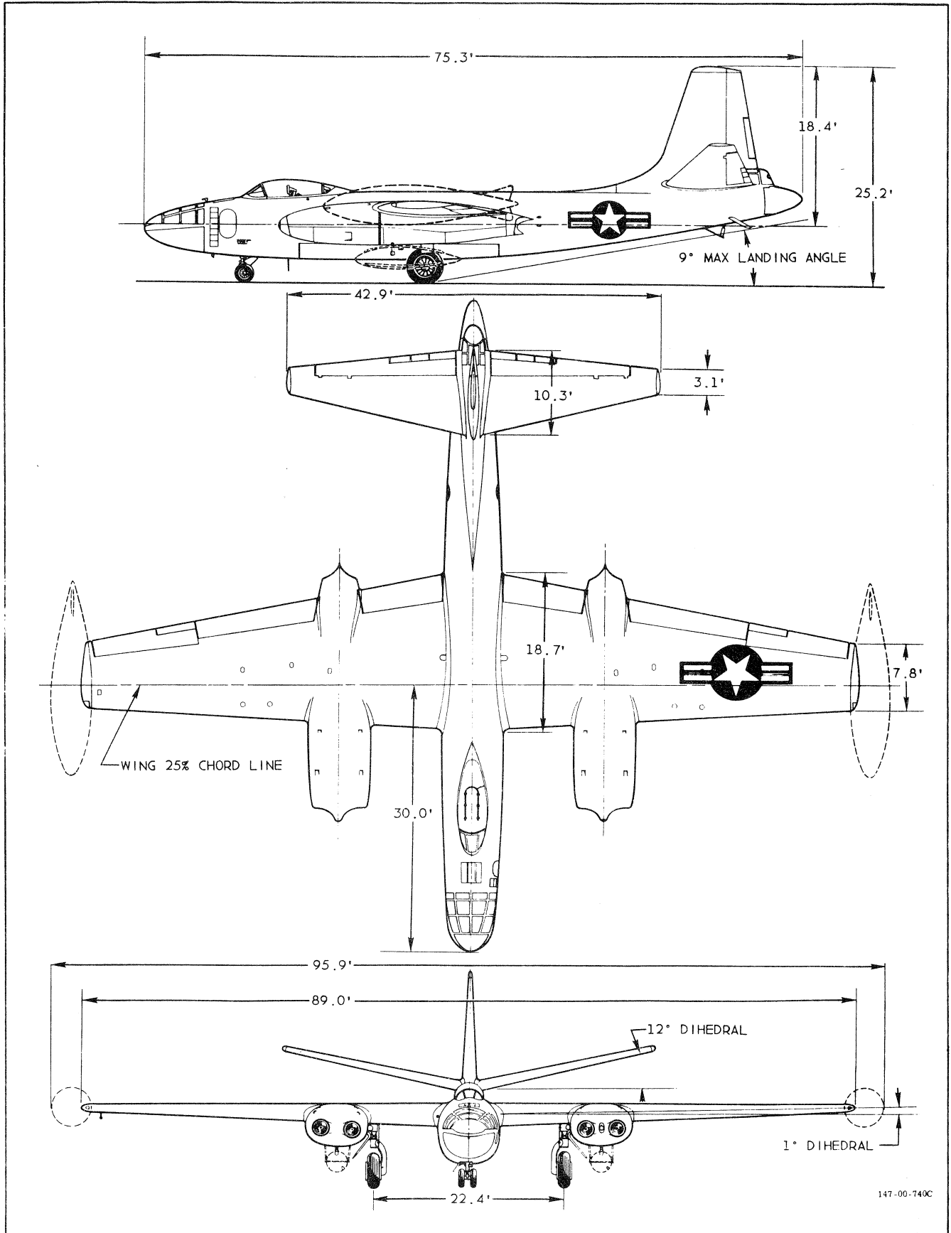
B-45A Figure 1-1. Airplane Dimensions
