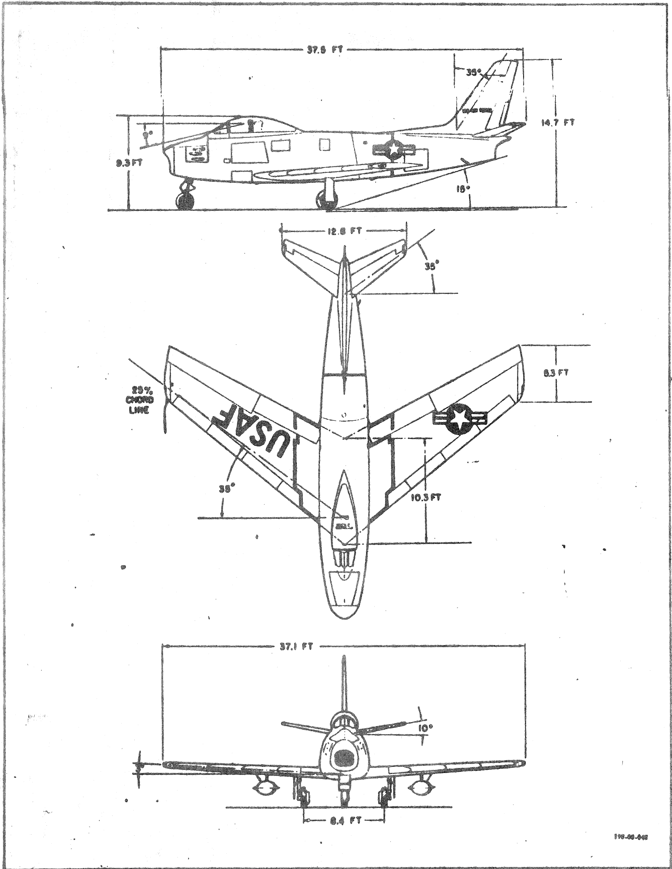
Figure 1-1. Airplane Dimensions
