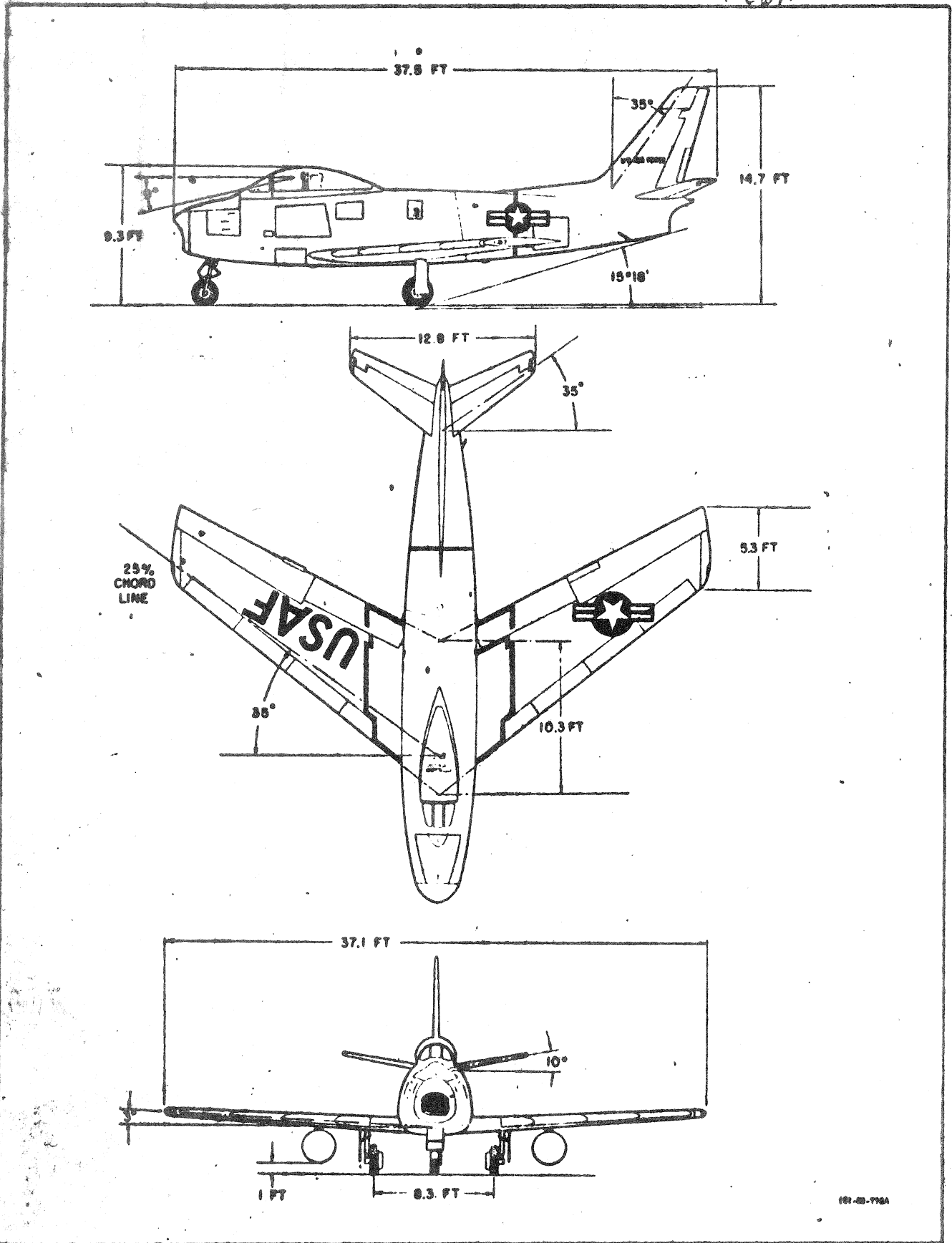
Figure 1-1. Airplane Dimensions
