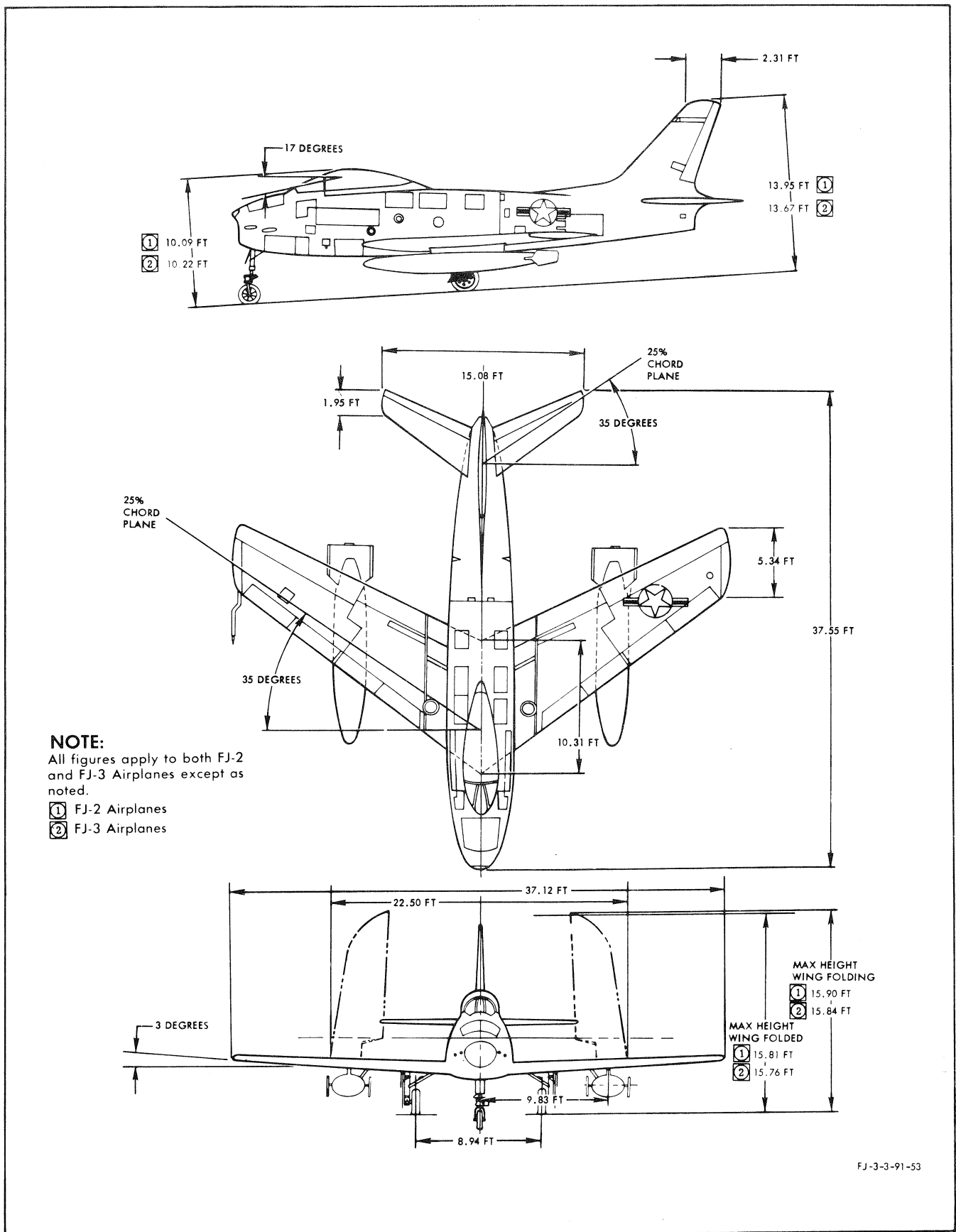
Figure 1-1. Airplane Dimensions - FJ-2 and FJ-3 Airplanes
