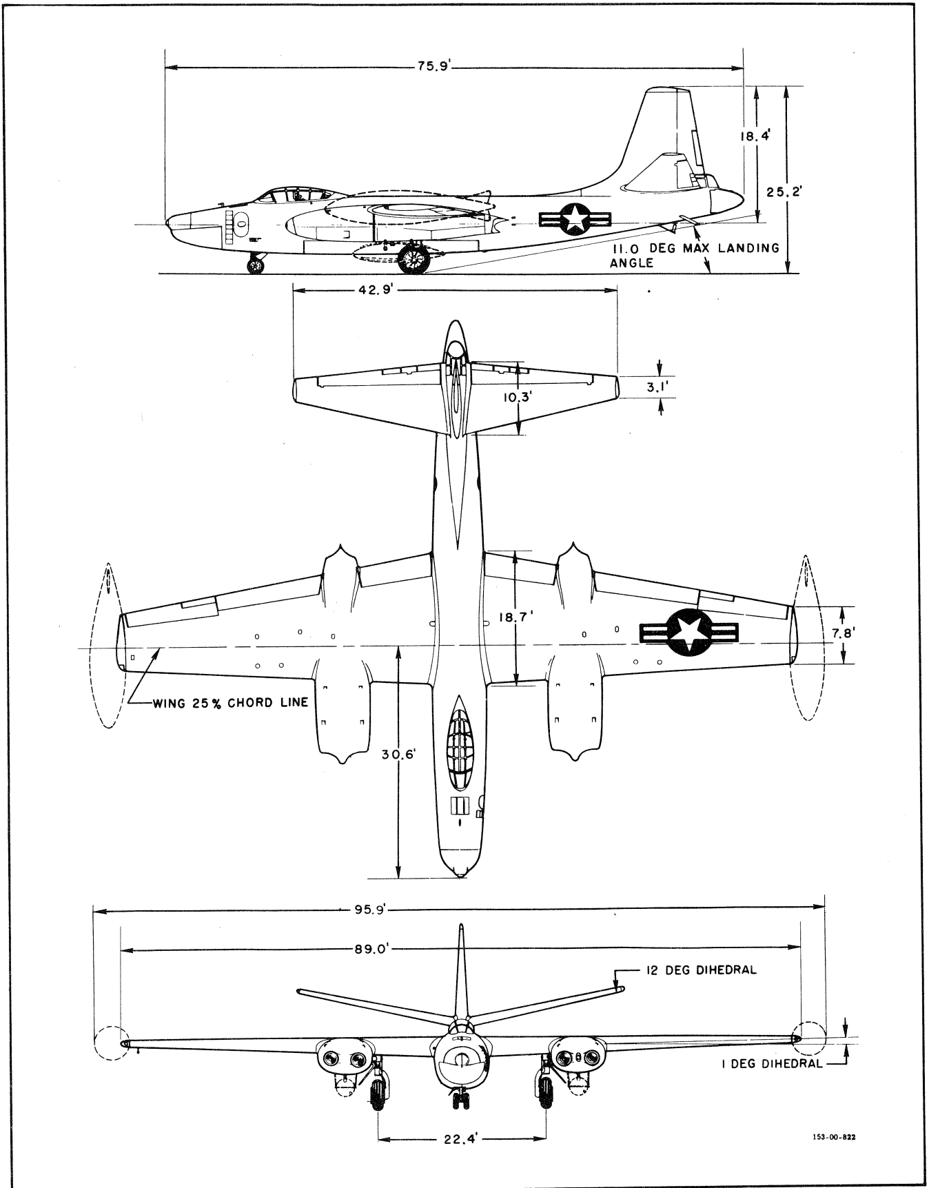
RB-45C Figure 1-1. Airplane Dimensions
