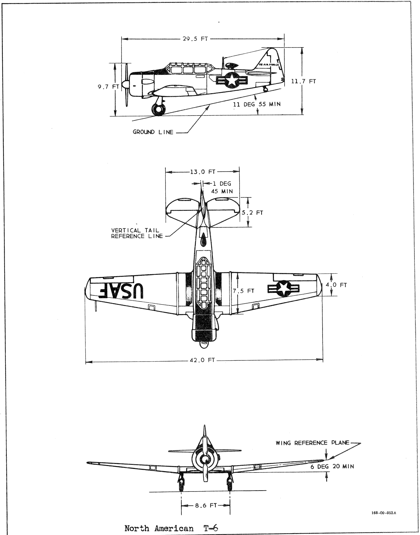
Figure 1-1. Principal Dimensions
