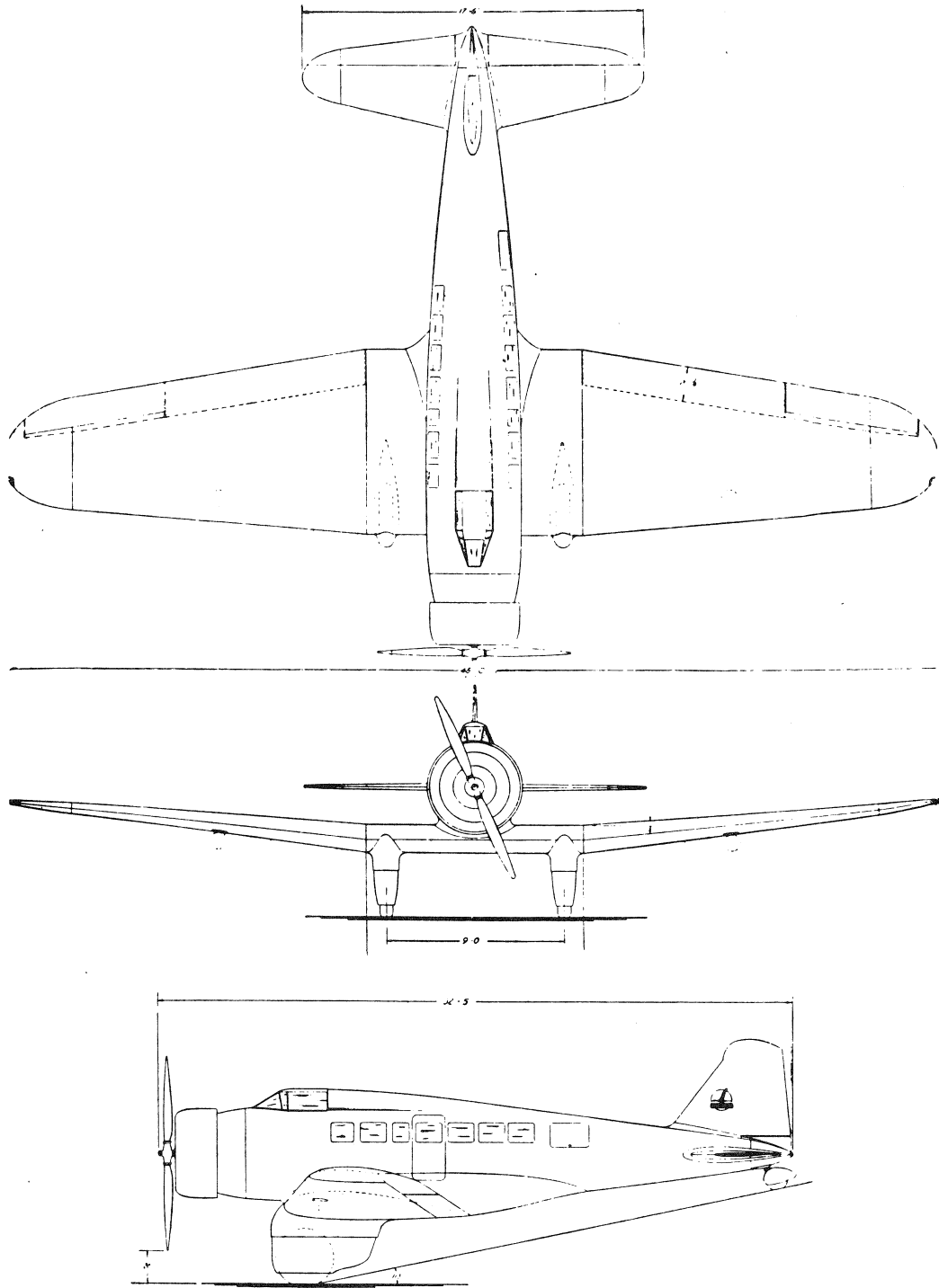
THE NORTHROP CORPORATION Inglewood, Calif. DELTA — 8 PLACE ENGINE: WRIGHT CYCLONE
