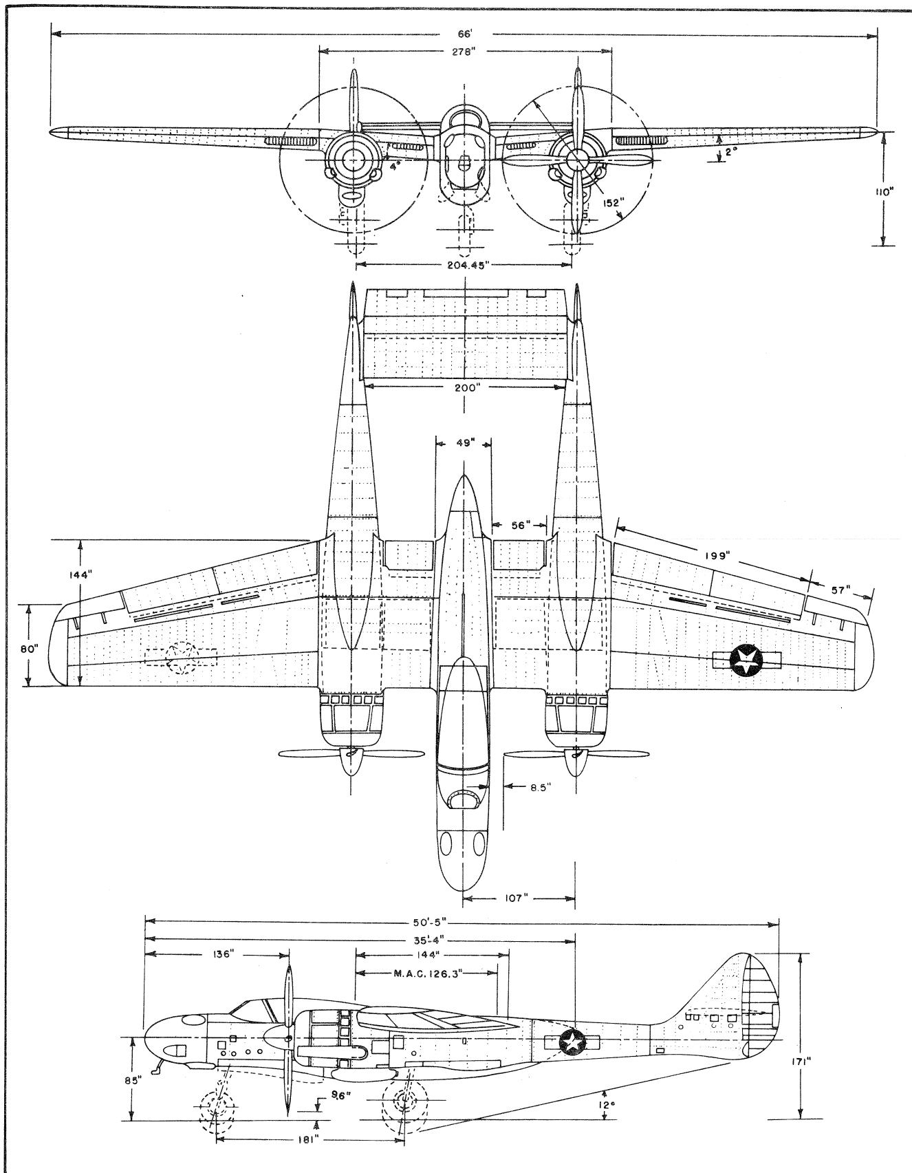
NORTHROP F-15A Figure 1-2 - Principal Dimensions
