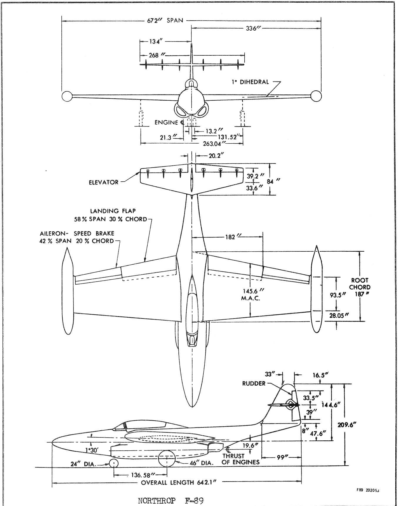
Figure 1-3. Principal Dimensions
